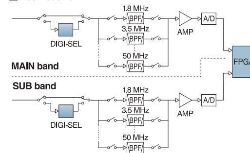
■ Dual receiver
